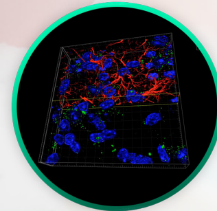
3D Reconstruction
